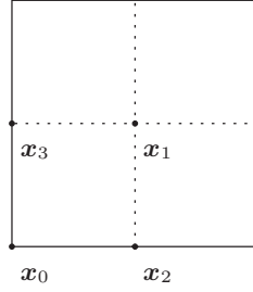
Figure 4.18 The four start points x_0, x_1, x_2, x_3 .
