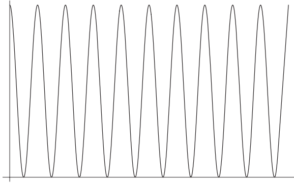
Figure 1.4 The function f(x) = \frac{c}{2N}(1 + \cos(2\pi Nx)) for N = 10 .
