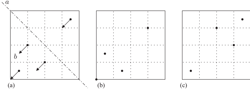
Figure 4.11 (0, 2, 2)-net in base 2 with elementary movements.
