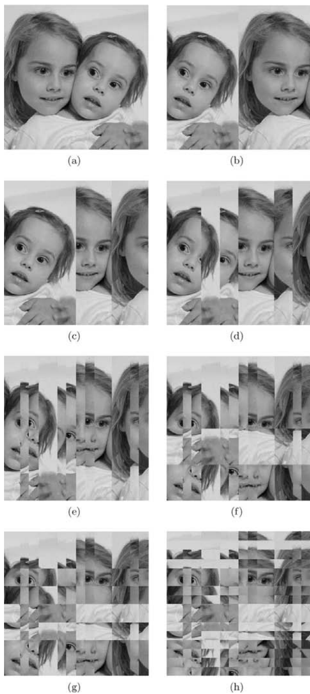
Figure 13.1 Owen's scrambling algorithm in base 2.
