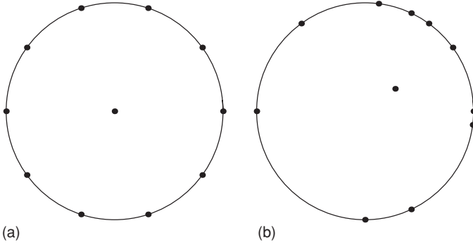
Figure 3.2 Ten points on the unit-circle. (a) The points are perfectly balanced and hence the centroid is exactly the origin. (b) For the points, the centroid is far away from the origin.
