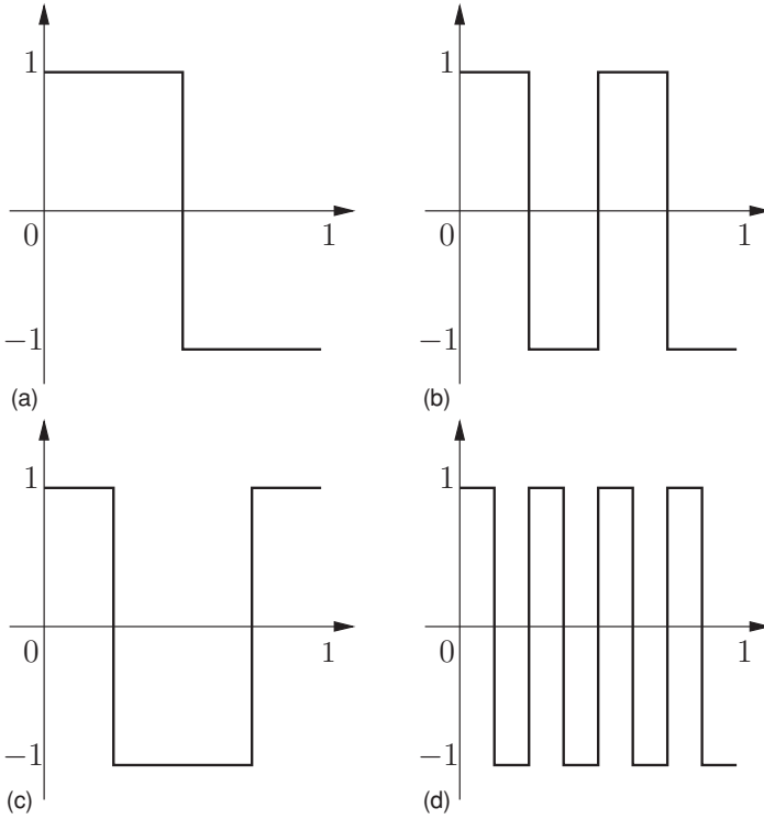
Figure 3.3 The 2-adic Walsh functions (a) {}_2\text{wal}_1(x) , (b) {}_2\text{wal}_2(x) , (c) {}_2\text{wal}_3(x) and (d) {}_2\text{wal}_4(x) .
