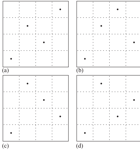
Figure 4.16 Four possible configurations for \mathbf{x}_0, \mathbf{x}_1, \mathbf{x}_2, \mathbf{x}_3 .
