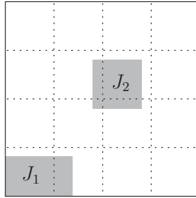
Figure 4.5 The intervals J_1 and J_2 .
