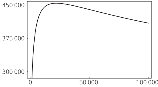
Figure 3.7 The function N \mapsto (\log N)^s / N for s = 10 .
