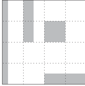
Figure 4.4 ‘Elementary’ intervals of area 1/16.
