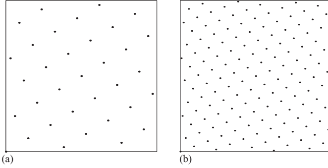
Figure 3.6 Two-dimensional lattice point sets with (a) N = 34 and \mathbf{g} = (1, 21) , and with (b) N = 144 and \mathbf{g} = (1, 89) .
