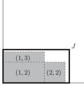
Figure 5.3 The set \underline{J} .
