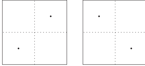
Figure 4.17 Configurations of two successive points.
