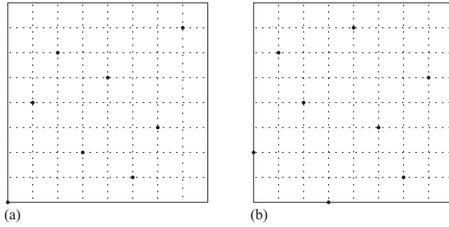
Figure 4.22 (a) A digital (0, 3, 2) -net over \mathbb{Z}_2 and (b) its digitally shifted version.
