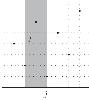
Figure 4.12 Projection of a (0, 3, 2) -net in base 2 to the first components.
