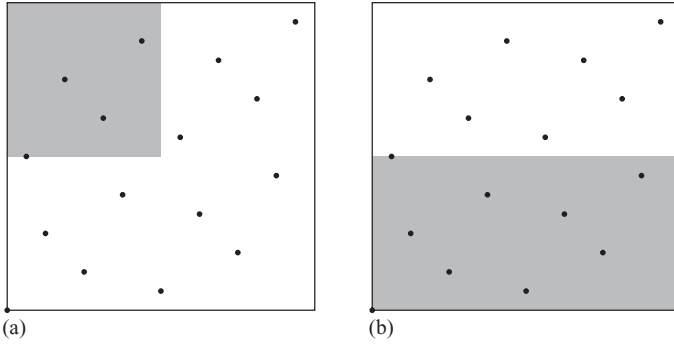
Figure 4.14 A (0, 4, 2) -net in base 2. The points in the elementary interval yield (a) a (0, 2, 2) -net in base 2 after doubling both coordinates; (b) a (0, 3, 2) -net in base 2 after doubling the second coordinate.
