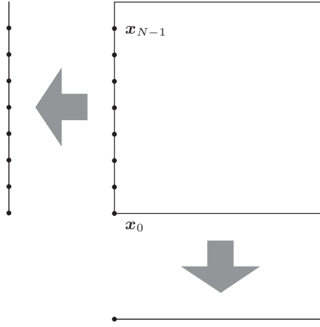
Figure 4.13 Projection of a (m, m, 2) -net to the first and second components.
