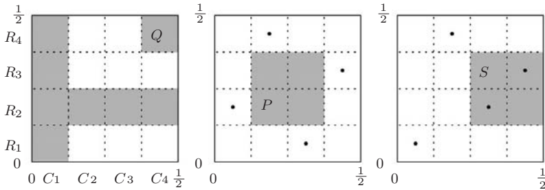
Figure 4.7 Placing four points in [0, 1/2]^2 which are fair with respect to R_1, R_2, R_3, R_4 and to C_1, C_2, C_3, C_4 .
